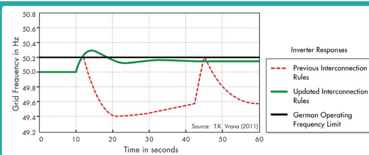
Figure 3: Example of Improved Performance with Inverter Controls That Implement a Droop Function for Over-Frequency Conditions Rather Than Tripping.
