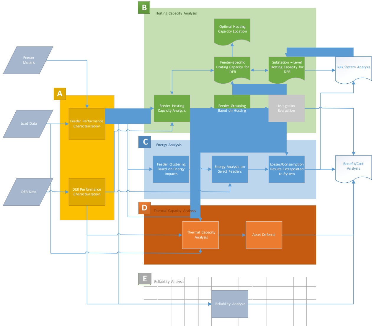
Figure 5-3 EPRI's Integrated Grid distribution analysis framework
