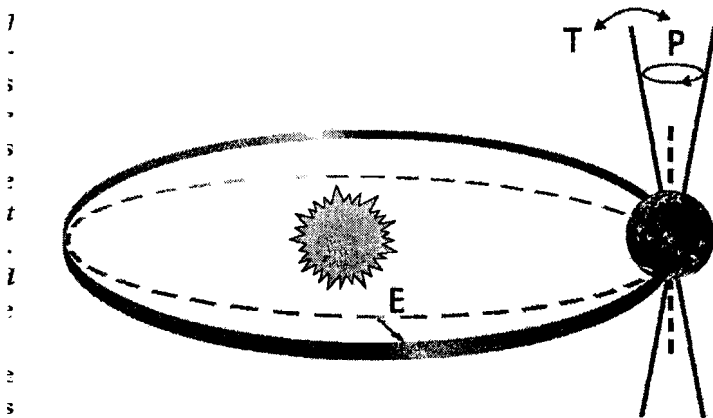
FAQ 6.1, Figure 1. Schematic of the Earth's orbital changes (Milankovitch cycles) that drive the ice age cycles. 'T' denotes changes in the tilt (or obliquity) of the Earth's axis, 'E' denotes changes in the eccentricity of the orbit (due to variations in the minor axis of the ellipse), and 'P' denotes precession, that is, changes in the direction of the axis tilt at a given point of the orbit. Source: Rahmstorf and Schellnhuber (2006).
