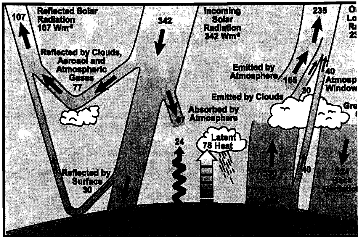
FAQ 1.1, Figure 1. Estimate of the Earth's annual and global mean energy balance. Over the long term, the amount of incoming solar radiation absorbed
