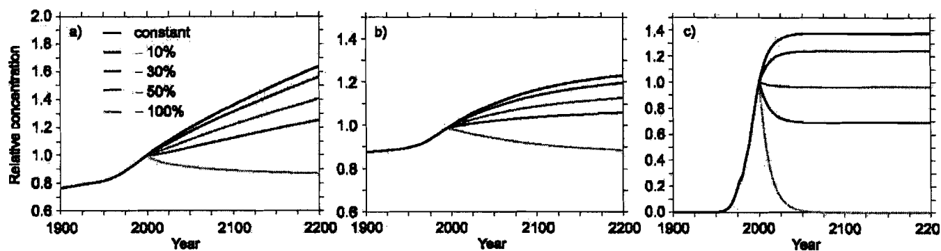
Figure 1. (a) Simulated changes in atmospheric CO 2 concentration relative to the present-day for emissions stabilised at the current level (black), or at 10% (red), 30% (green), 50% (dark blue) and 100% (light blue) lower than the current level; (b) as in (a) for a trace gas with a lifetime of 120 years, driven by natural and anthropogenic fluxes; and (c) as in (a) for a trace gas with a lifetime of 12 years, driven by only anthropogenic fluxes.
