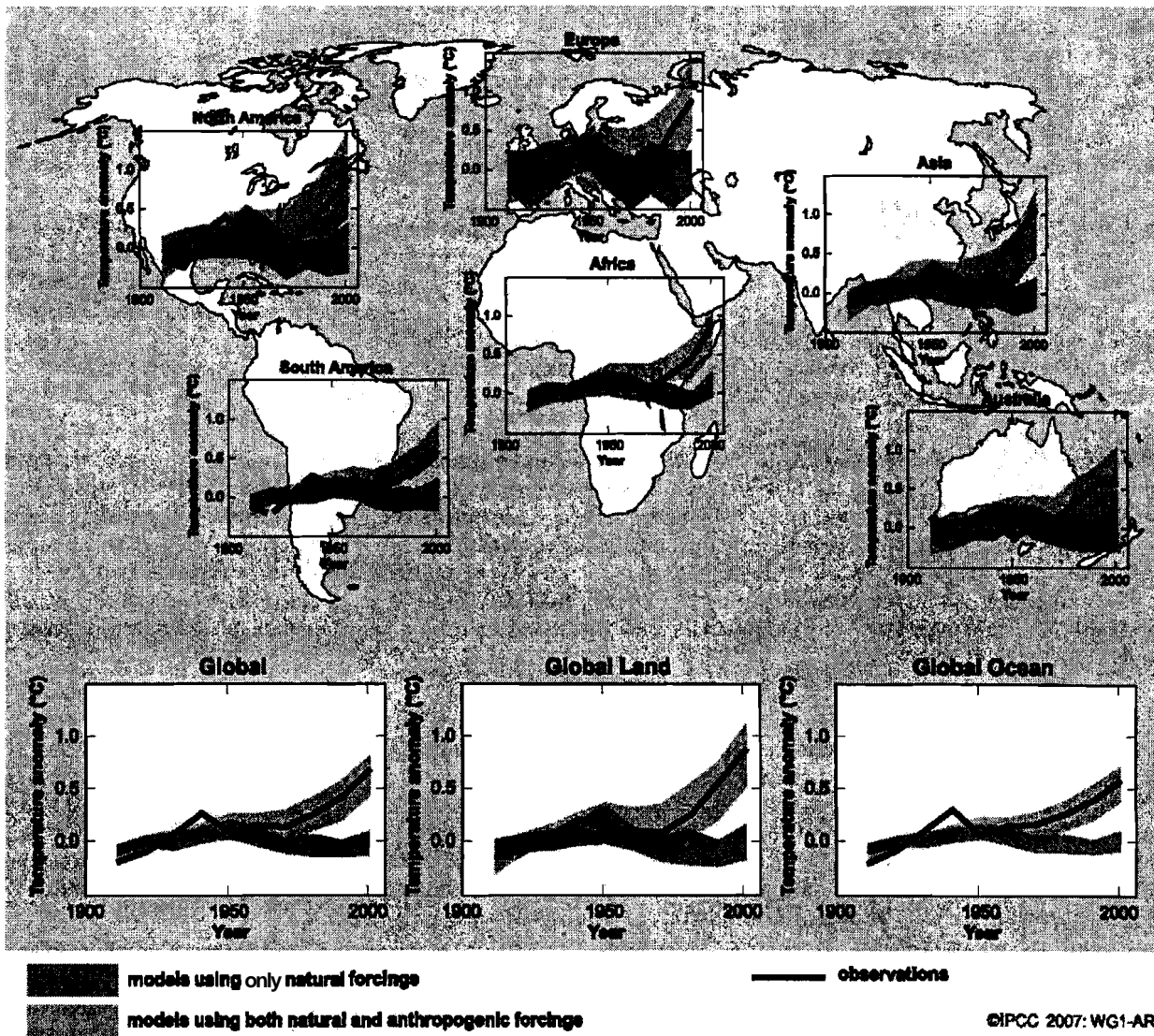
FAQ 9.2, Figure 1. Temperature changes relative to the corresponding average for 1901-1950 ( ^{\circ}\text{C} ) from decade to decade from 1906 to 2005 over the Earth's continents, as well as the entire globe, global land area and the global ocean (lower graphs). The black line indicates observed temperature change, while the coloured bands show the combined range covered by 90% of recent model simulations. Red indicates simulations that include natural and human factors, while blue indicates simulations that include only natural factors. Dashed black lines indicate decades and continental regions for which there are substantially fewer observations. Detailed descriptions of this figure and the methodology used in its production are given in the Supplementary Material, Appendix 9.C.
